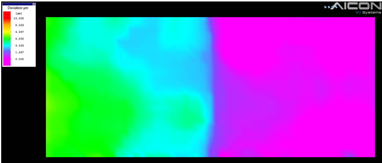
Fig. 4: figure provided with courtesy by Mr. Hermstein, AICON 3D Systems GmbH measuring of layer thickness on a scanned object after application of ReflexEx.
